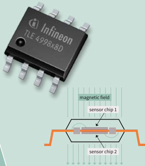
The Dual Hall Sensor TLE4998 includes two sensor ICs which are placed exactly on top of each other. This kind of redundancy is a basic requirement for highly dependable systems.
