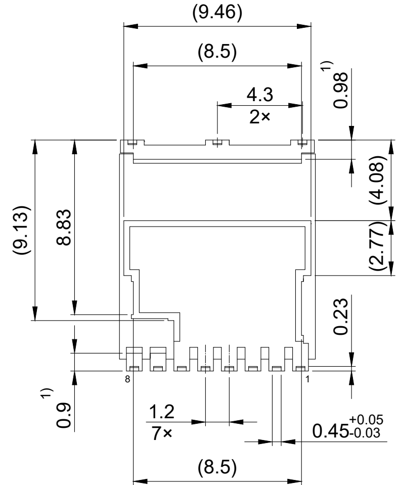
Bottom view
