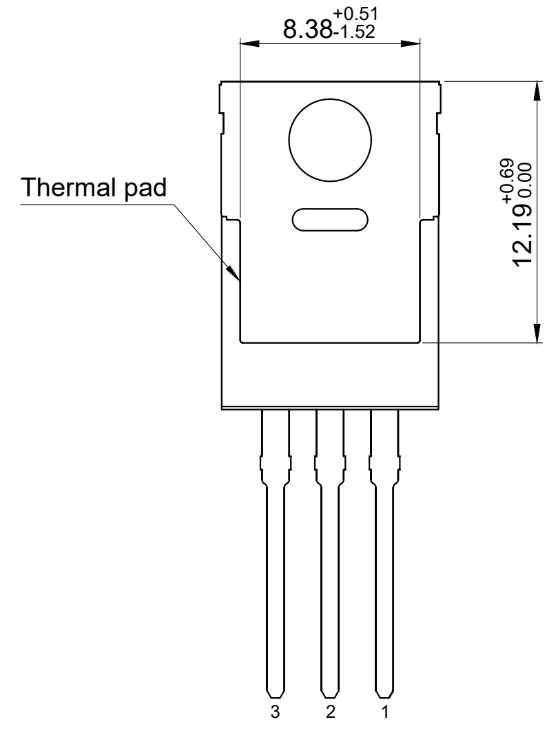
Bottom view
