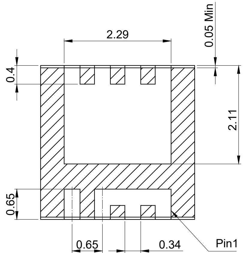
Bottom view
