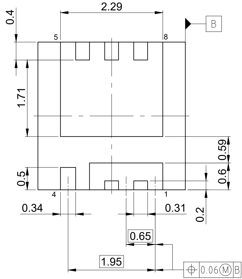
Bottom View
