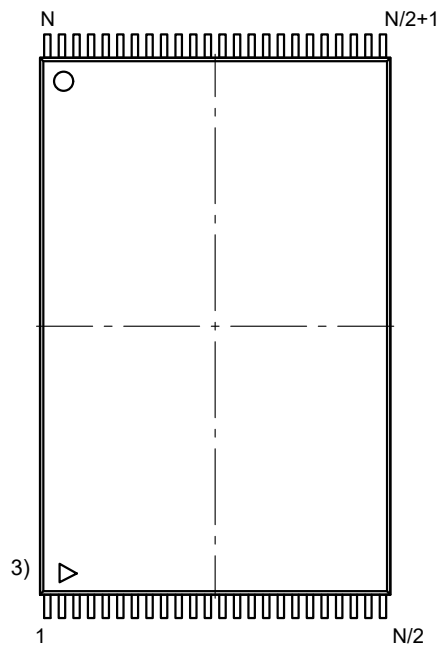
Reverse pin out (top view)
