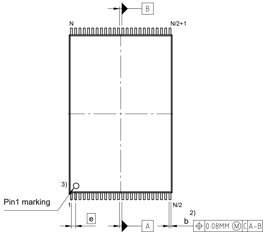
Standard pin out (top view)
